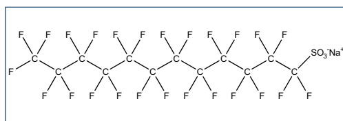
Sodium Perfluoro-1-dodecanesulfonate
