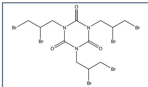
Tris(2,3-dibromopropyl)isocyanurate (T23BPIC)
